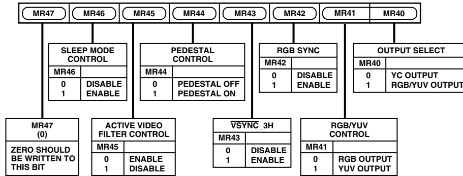
Figure 29. Mode Register 4
