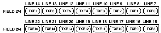
Figure 36. Teletext Control Registers
