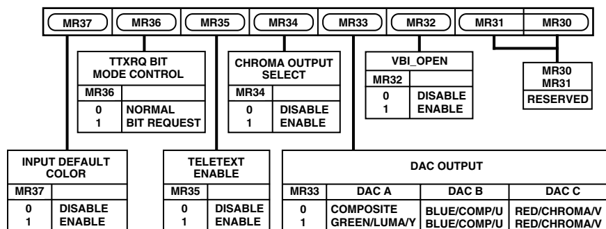
Figure 28. Mode Register 3
