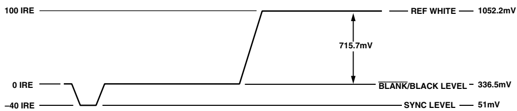
Figure 55. NTSC RGB Video Levels
