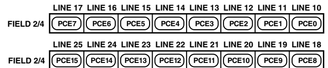
Figure 35. Pedestal Control Registers
