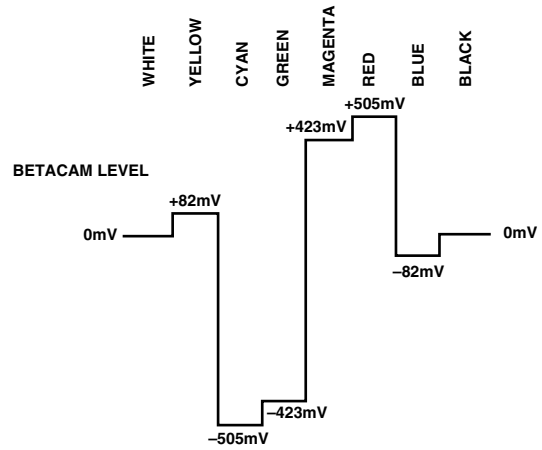
Figure 63. NTSC 100% Color Bars, No Pedestal V Levels
