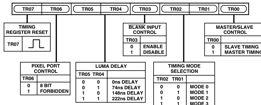
Figure 30. Timing Register 0
