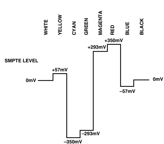
Figure 64. NTSC 100% Color Bars with Pedestal V Levels
