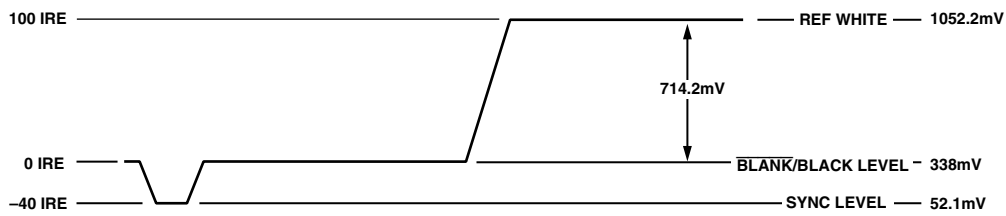
Figure 53. NTSC Luma Video Levels
