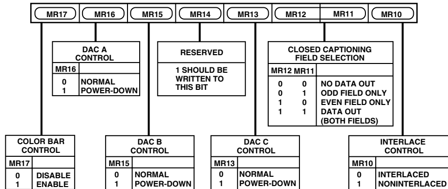
Figure 26. Mode Register 1
