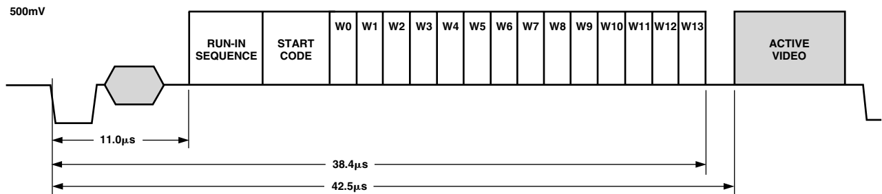
Figure 45. WSS Waveform Diagram
