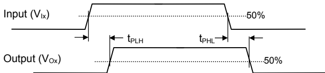
Figure 3. Propagation Delay Parameters.
