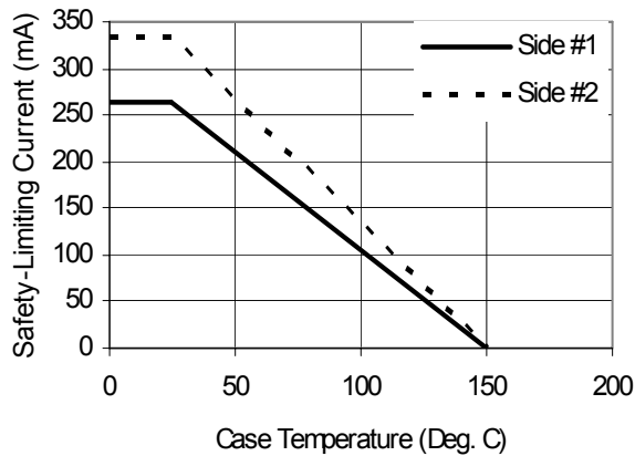
Figure 1. Thermal Derating Curve, Dependence of Safety Limiting Values with Case Temperature per DIN EN 60747-5-2.
