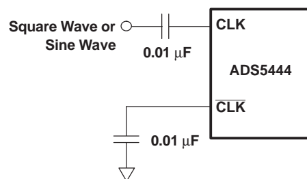
Figure 37. Single-Ended Clock
