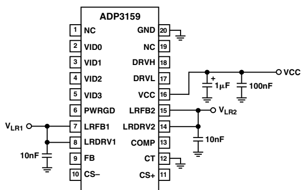
Figure 2. Linear Regulator Output Voltage Accuracy Test Circuit
