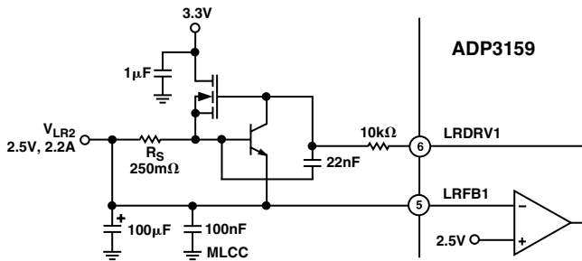
Figure 6. Adding Overcurrent Protection to the Linear Regulator
