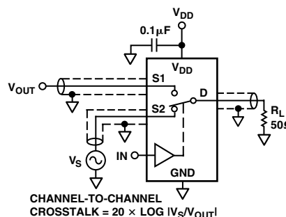
Test Circuit 7. Channel-to-Channel Crosstalk CHANNEL-TO-CHANNEL CROSSTALK = 20 \times \log |V_S/V_{OUT}|
