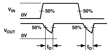
Test Circuit 5. Break-Before-Make Time Delay, t_D
