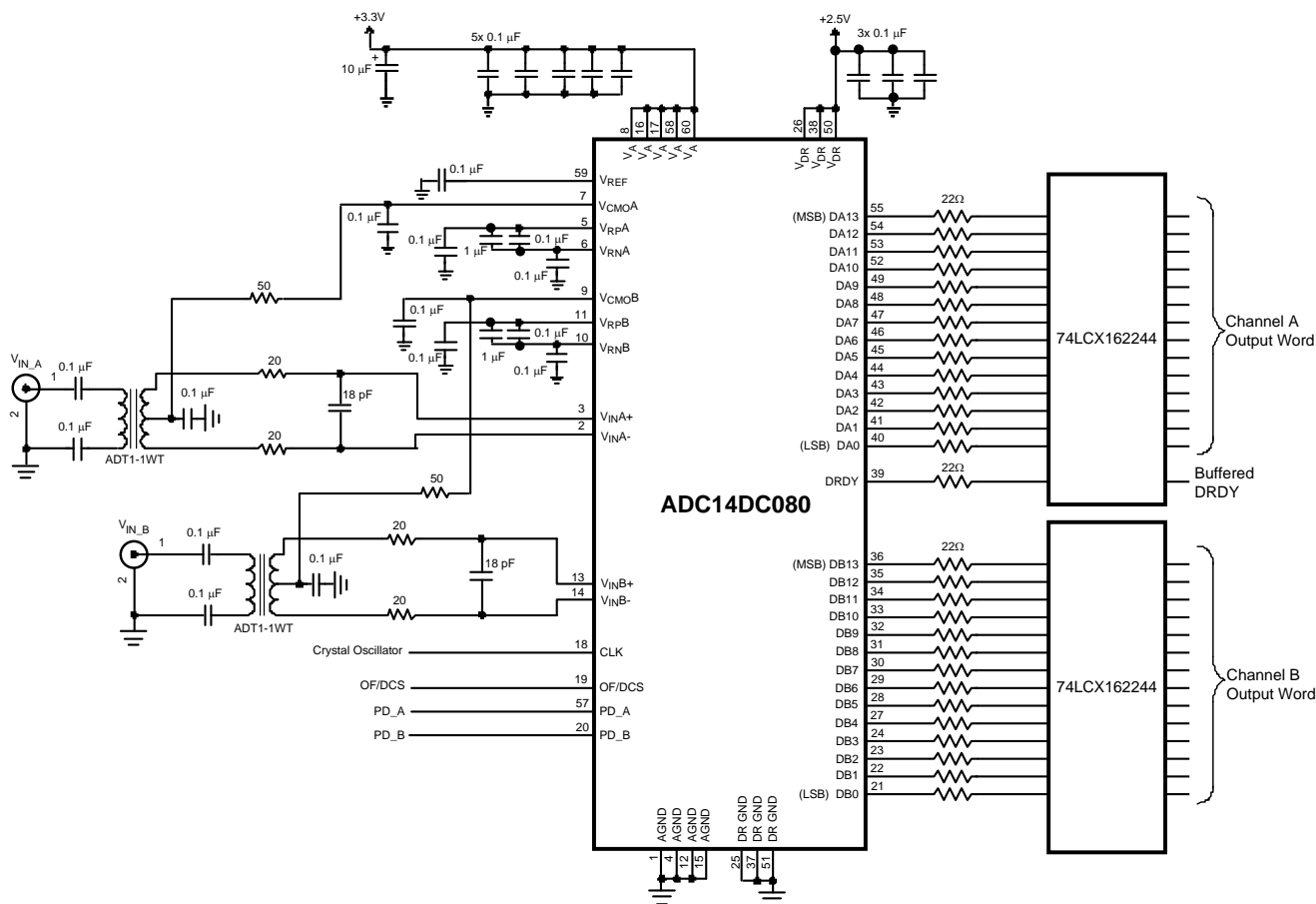
Figure 21. Application Circuit
