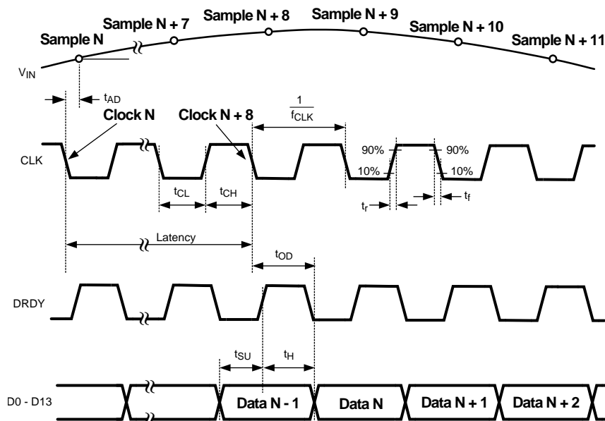
Figure 2. Output Timing
