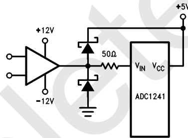
Protecting the Analog Inputs
