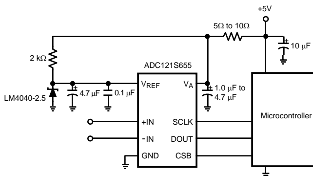
Figure 61. Low cost, low power Data Acquisition System
