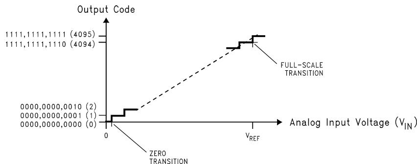
Figure 1. Transfer Characteristic
