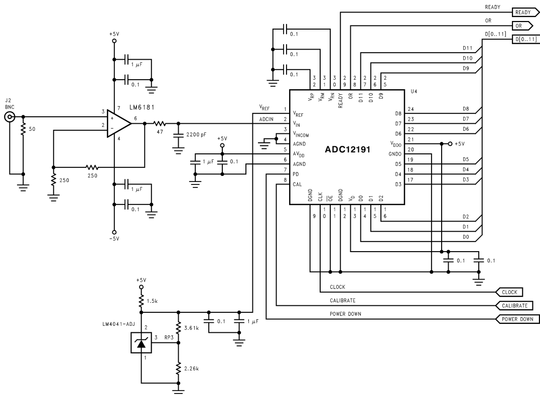
Figure 5. Basic Connections Diagram
