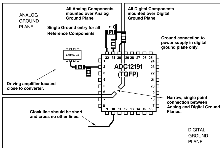
Figure 6. Layout example
