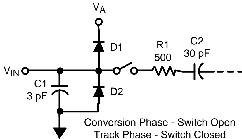
Figure 50. Equivalent Input Circuit
