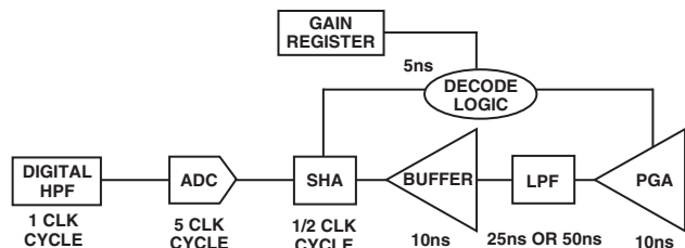
Figure 4. AGC Timing
