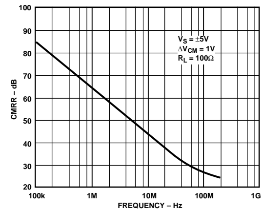
Figure 44. AD9632 CMRR vs. Frequency
