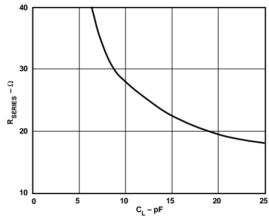
Figure 61. Recommended R_{SERIES} vs. Capacitive Load
