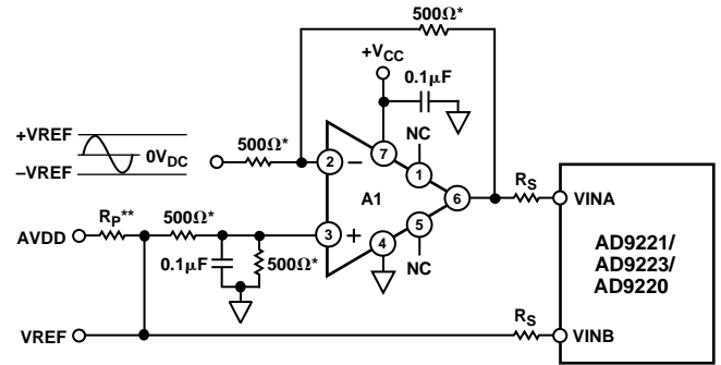
Figure 40. Single-Ended Input With DC-Coupled Level Shift
