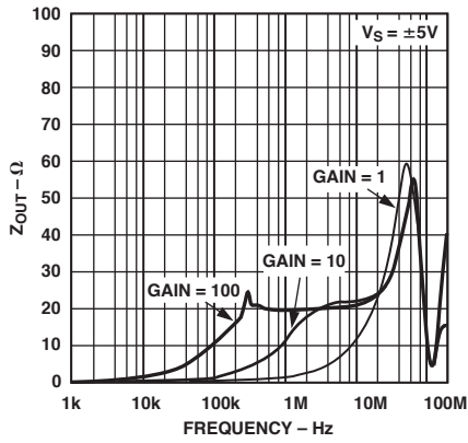
TPC 28. Z_{OUT} vs. Frequency
