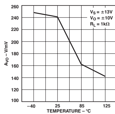
TPC 17. A_{VO} vs. Temperature at \pm 13\text{ V}
