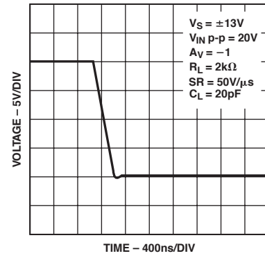
TPC 38. -SR at G = -1
