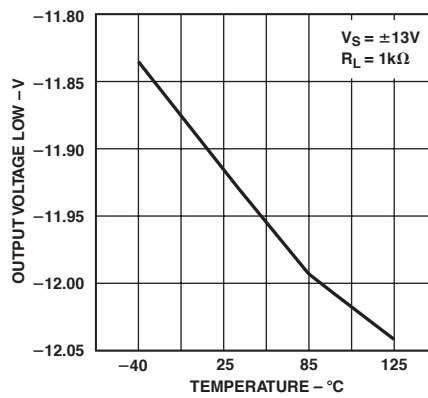
TPC 14. Output Voltage Low vs. Temperature at \pm 13\text{ V}
