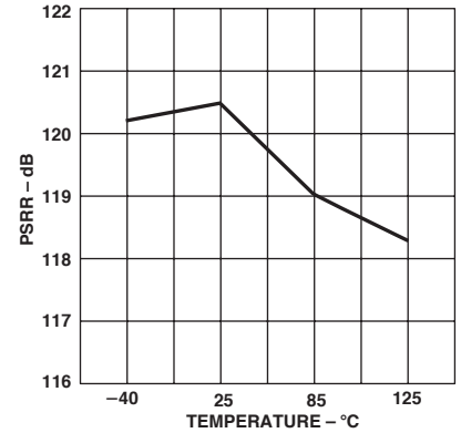
TPC 21. PSRR vs. Temperature
