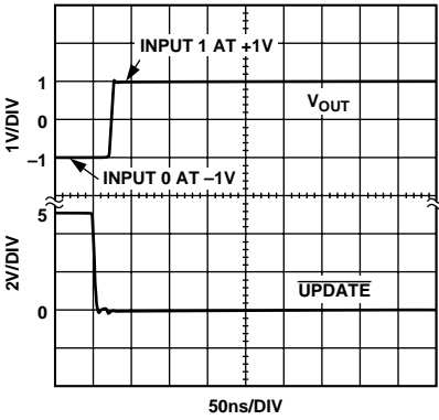
Figure 33. AD8110 Switching Time
