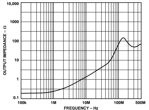
Figure 23. AD8110 Output Impedance, Enabled
