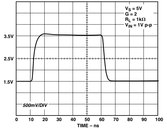
TPC 34. 1 V Step Response
