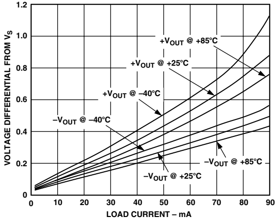
TPC 1. Output Saturation Voltage vs. Load Current
