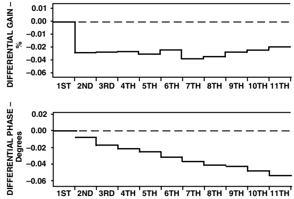
TPC 16. Differential Gain and Phase Error, G = 2 , NTSC Input Signal, R_L = 1 k\Omega , V_S = 5 V
