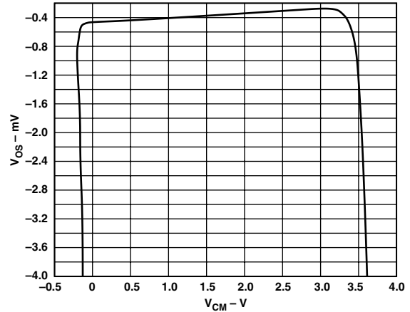
Figure 3. V_{OS} vs. Common-Mode Voltage, V_S = 5 V
