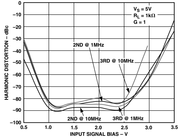
TPC 10. Harmonic Distortion for a 1 V p-p Signal vs. Input Signal DC Bias
