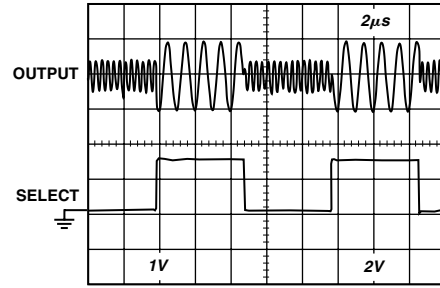
Figure 15. AD8063 Mux Output
