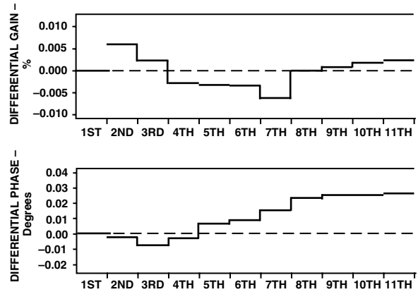
TPC 17. Differential Gain and Phase Error, G = 2 , NTSC Input Signal, R_L = 150 \Omega , V_S = 5 V
