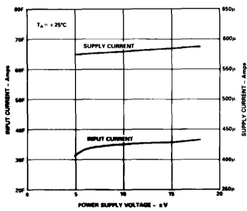
Figure 7. Input Bias Current and Supply Current vs. Supply Voltage
