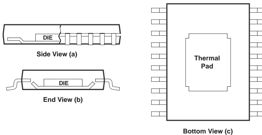
Figure 25. Views of Thermally Enhanced PWP Package
