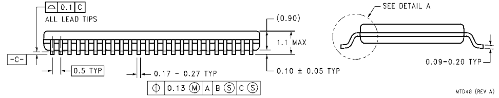
48-Lead Thin Shrink Small Outline Package (TSSOP), JEDEC MO-153, 6.1mm Wide Package Number MTD48
