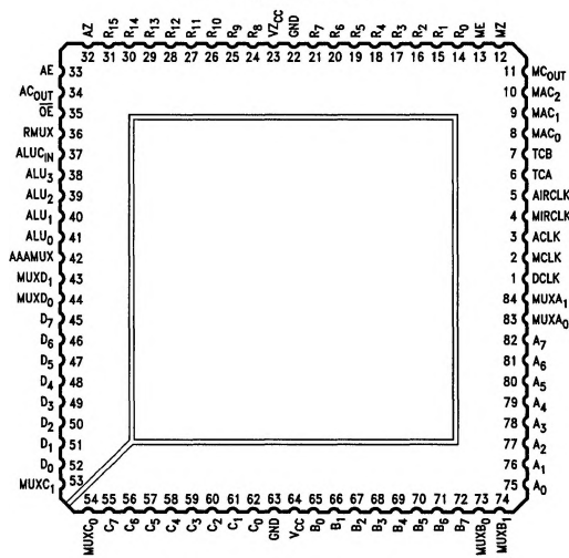
Pin Assignment for PCC
