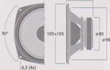
SP-60/8
